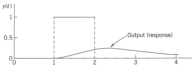
Fig. 143. Square wave and response in Example 5
