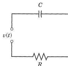
Fig. 124. RC -circuit, electromotive force v(t) , and current in Example 3
