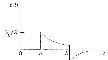
Fig. 124. RC -circuit, electromotive force v(t) , and current in Example 3
