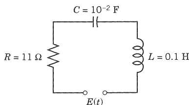
Fig. 125. RLC -circuit in Example 4
