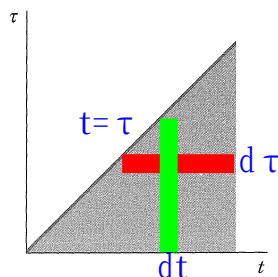
Fig. 141. Region of integration in the t\tau -plane in the proof of Theorem 1
